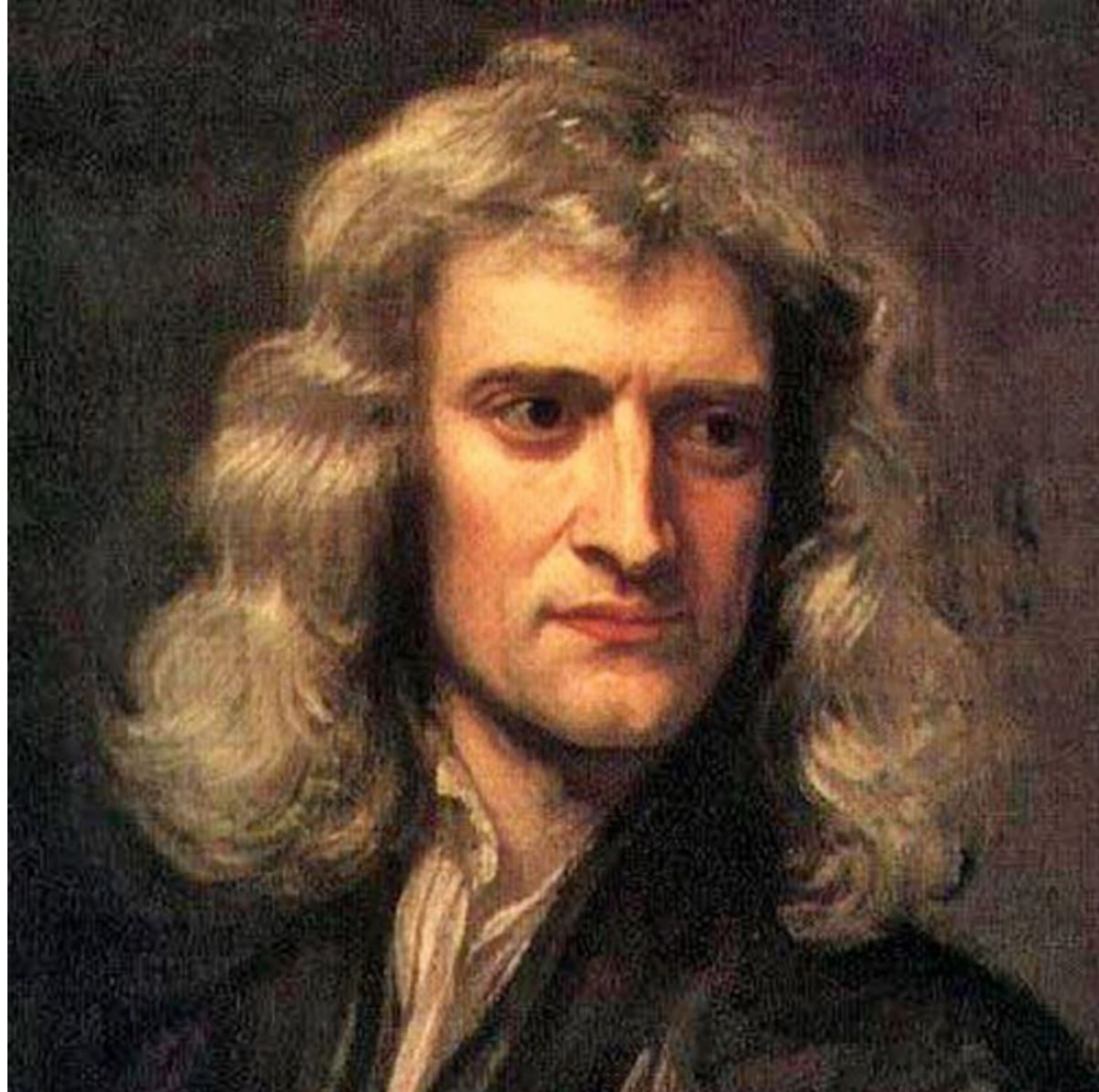
Gravity
